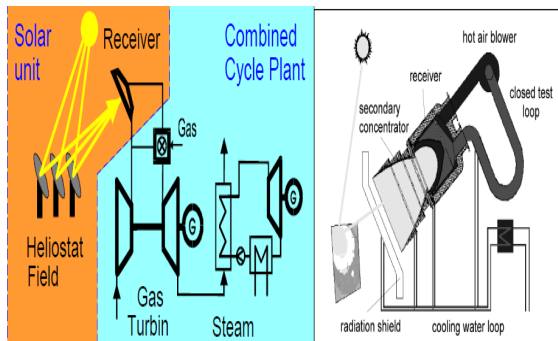
Figure 4. The REFOS-receiver for testing at the Plataforma Solar de Almería. Source:[23]
