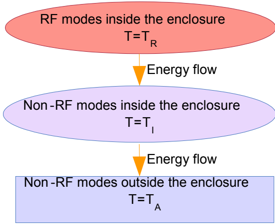
Figure 3. The thought experiment with thermally conducting enclosure wall - the three subsystems in Local Thermodynamic Equilibrium (LTE)
