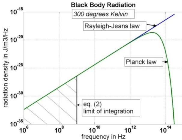
Figure 1. Black body radiation spectra at 300 0 K. The shaded area is integrated over in eq. (2)
